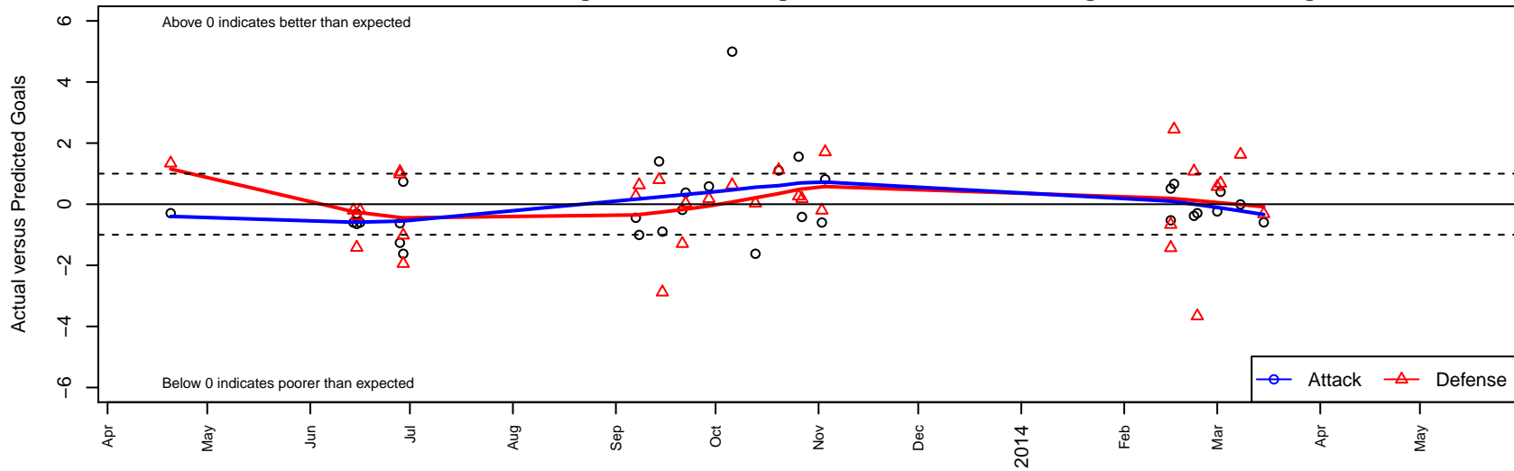
THUSC Argon B99 Dots are actual minus expected GF (blue circles) and GA (red triangles). Blue line is smoothed change in attack strength. Red is smoothed change in defense strength.
